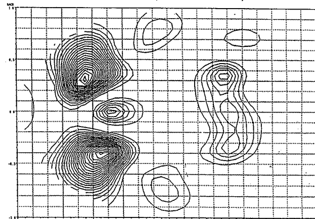
Fig. 4. Surface energy density (SED). Leftmost axis represents back of the head, right axis represents front of the head. Top row is the SED on the left and its contour map for the primed non-famous face. The greatest energy is located at the temporal sites with emphasis on the right temporal region. Bottom row illustrates the SED and its contour for the energy involved in processing the recognition of famous faces. Note the energy at the temporal region with additional involvement of the frontal region.
