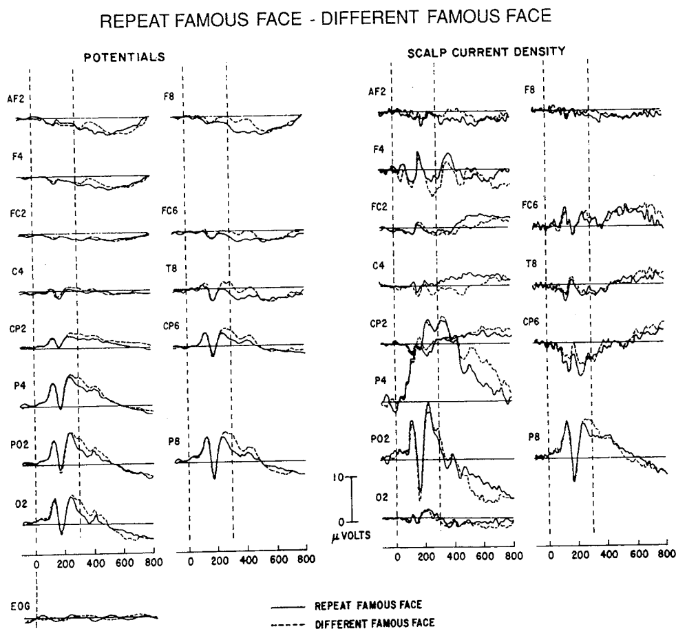
Fig. 1. Grand mean ERP wave form: repeat famous face and different famous face. Left two columns illustrate potential recordings; right two columns reflect the same data transformed as scalp current density. In this experiment a downward deflection indicates greater negativity at the most posterior electrodes with respect to the vertex (Cz) electrode.
