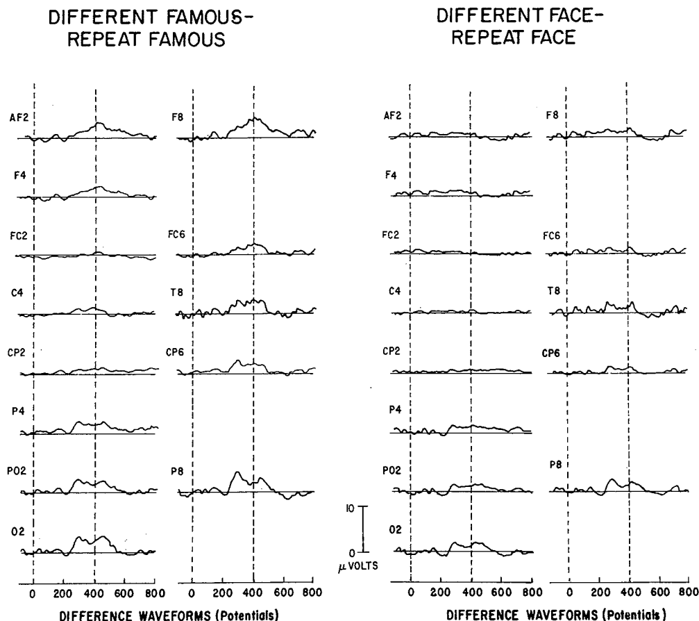
Fig. 3. Difference wave forms obtained by subtracting scalp potentials between different famous faces minus repeat famous faces (left columns), and different non-famous faces minus repeat non-famous faces (right columns).
