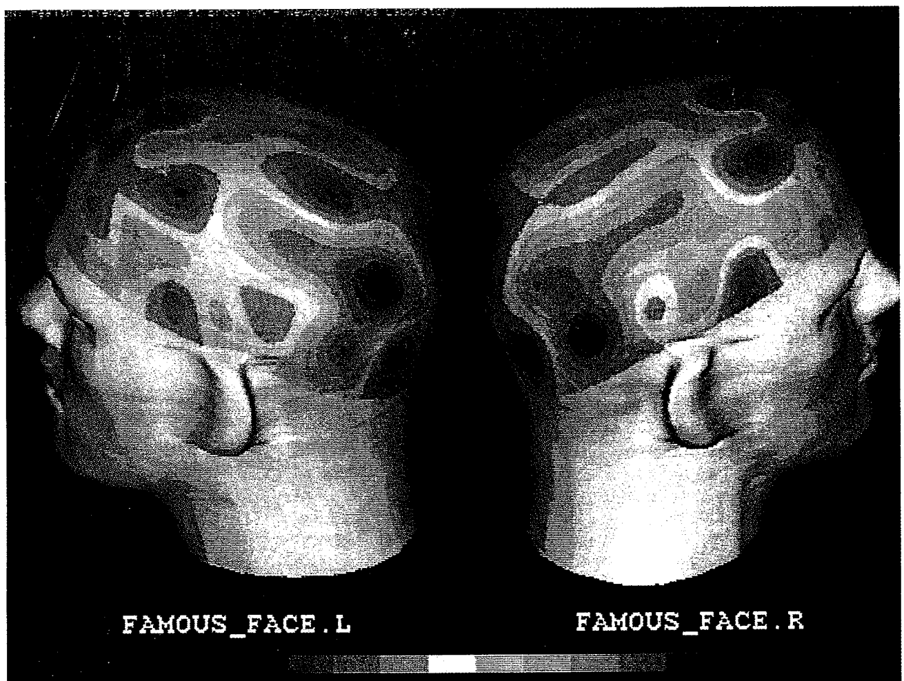
Fig. 5. Current source density map, VMP-C4 component. Source is represented by red, the sink by blue.
