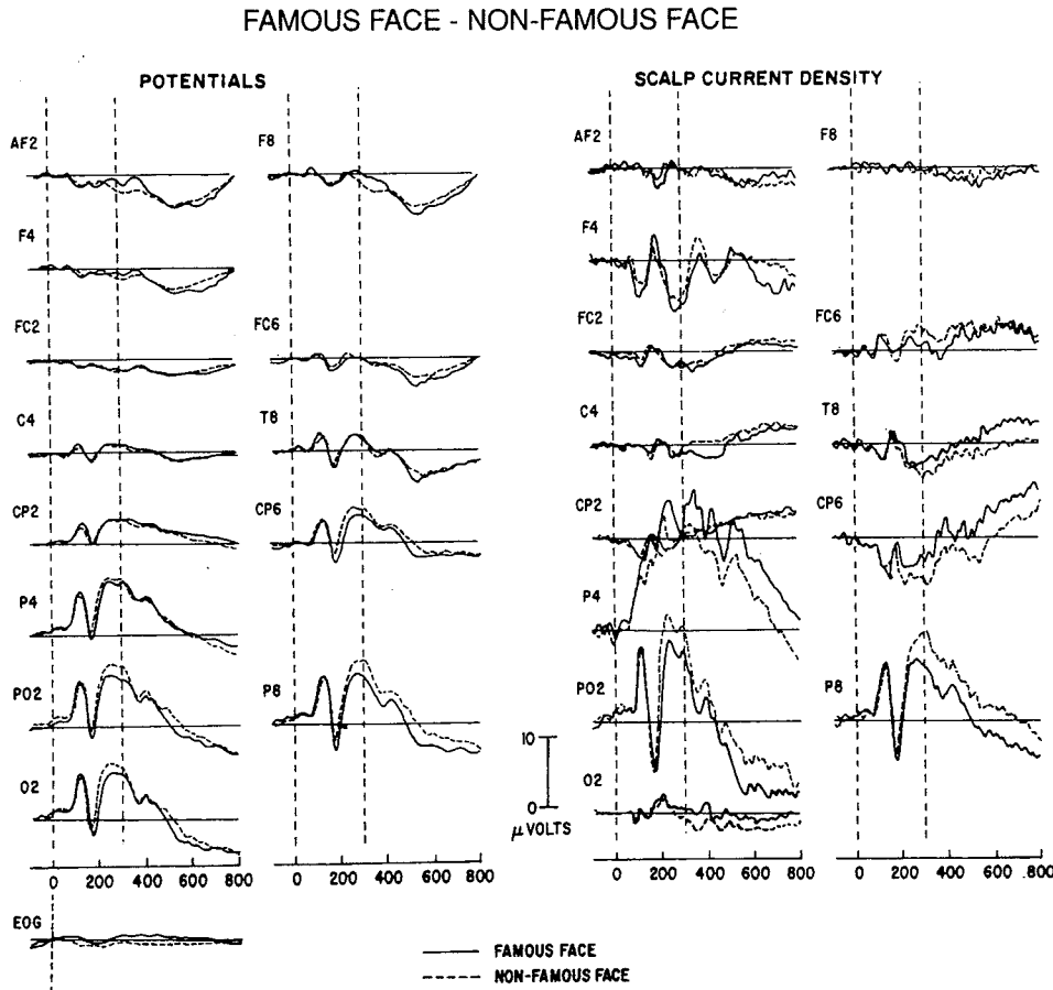
Fig. 2. Grand mean ERP wave form: famous face and non-famous face. Left two columns and right two columns same as in Fig. 1. Polarity same as in Fig. 1.
