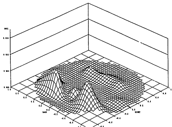
Fig. 4. Surface energy density (SED). Leftmost axis represents back of the head, right axis represents front of the head. Top row is the SED on the left and its contour map for the primed non-famous face. The greatest energy is located at the temporal sites with emphasis on the right temporal region. Bottom row illustrates the SED and its contour for the energy involved in processing the recognition of famous faces. Note the energy at the temporal region with additional involvement of the frontal region.
