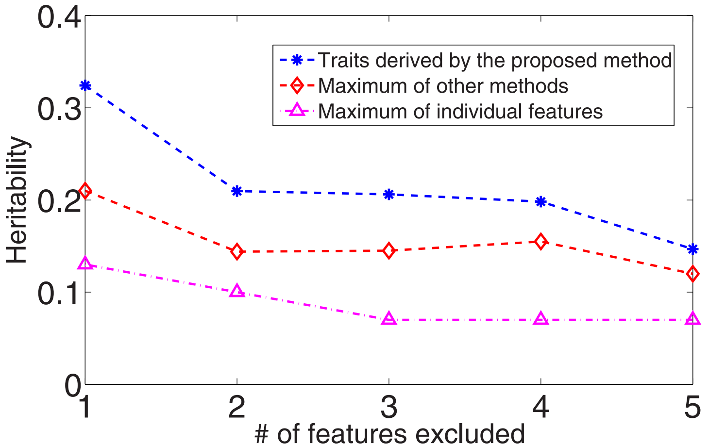
Fig 5. Heritability comparison between the traits derived by the proposed approach, by other methods, and original features when relevant features were randomly selected and excluded from the training data.
