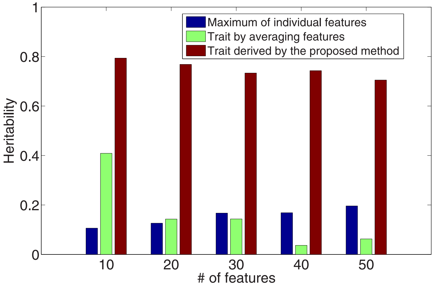
Fig 3. Heritability comparison between the trait derived by the proposed approach, individual features and the simple average of features (without covariate effects).
