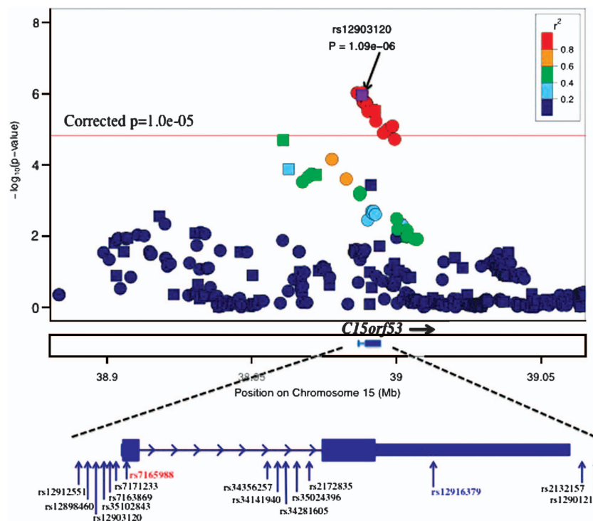
Figure 3. Plot of chromosome 15q14 association with DSM-IV alcohol-dependence SC. Squares represent genotyped SNPs; circles represent imputed SNPs. SNP rs7165988 (in red) is a non-synonymous coding variant. SNP rs12916379 (in blue) is in 3' untranslated region of C15orf53 .
