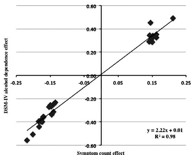
Figure 4. Correlation between symptom-count effect and DSM-IV alcohol-dependence effect in COGA sample.
