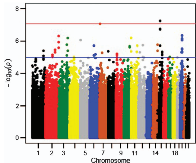
Figure 2. Manhattan plot of genome-wide association results for DSM-IV alcohol-dependence SC using negative binomial analysis. -\log_{10} values shown here were not corrected for inflation factor.
