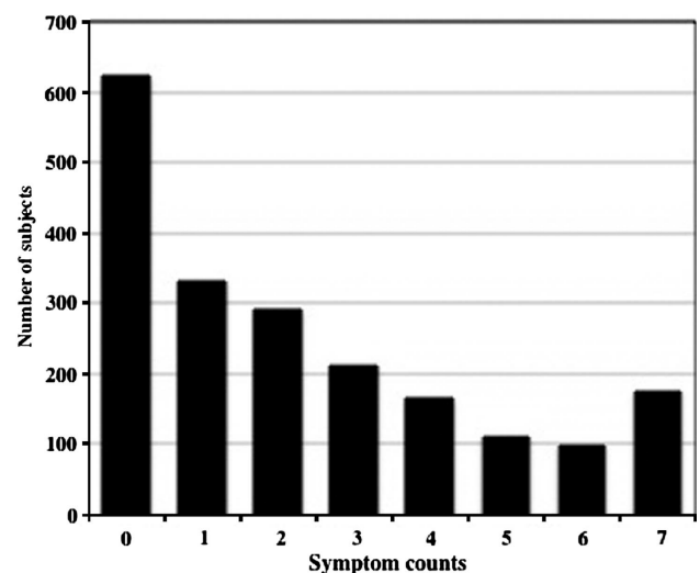
Figure 1. Distribution of DSM-IV alcohol-dependence symptom counts in the genotyped GWAS sample.
